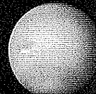
Neptune
