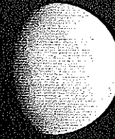
Mercury
